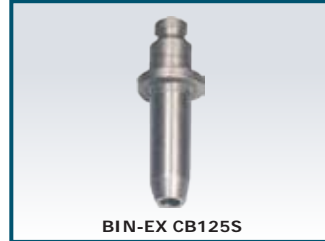
BIN-EX CB125S HONDA : CB100-125S P/No. 12021-107-310 (IN) 12023-107-310 (EX)
